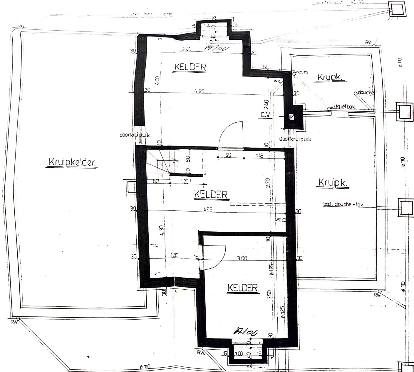
PLAN Kelder-Fundering-RIOLERING.
